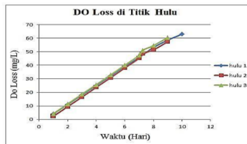
Gambar 3. DO Loss Segmen Hulu
