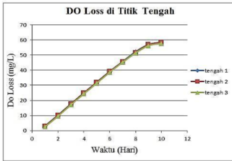
Gambar 4. DO Loss Segmen Tengah
