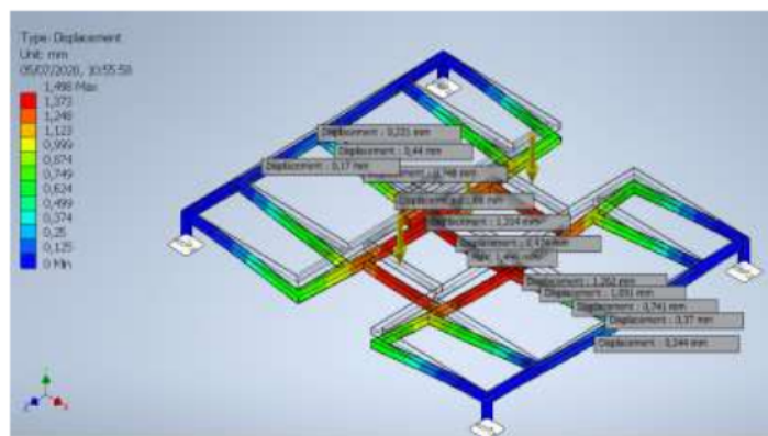
Gambar 4. Simulation Displacement
