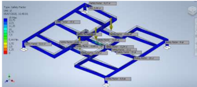
Gambar 8. Simulation Safety Factor
