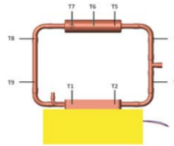
Fig. 5 Thermocouples placement
