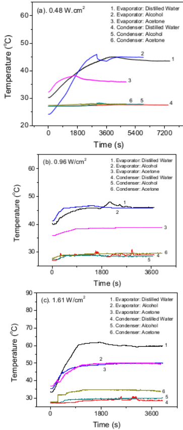
Fig. 8 Transient temperature history
