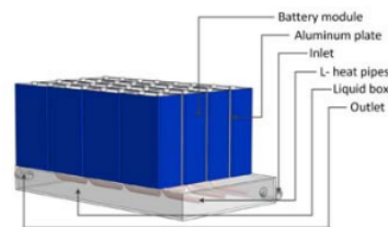
Fig. 1 Thermal management system of electric vehicle battery [15]
