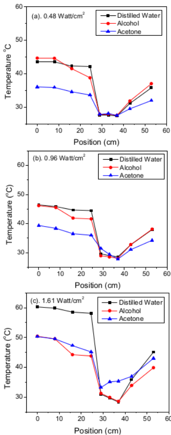
Fig. 9 Steady state temperature distribution
