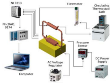
Fig. 7 Experimental setup
