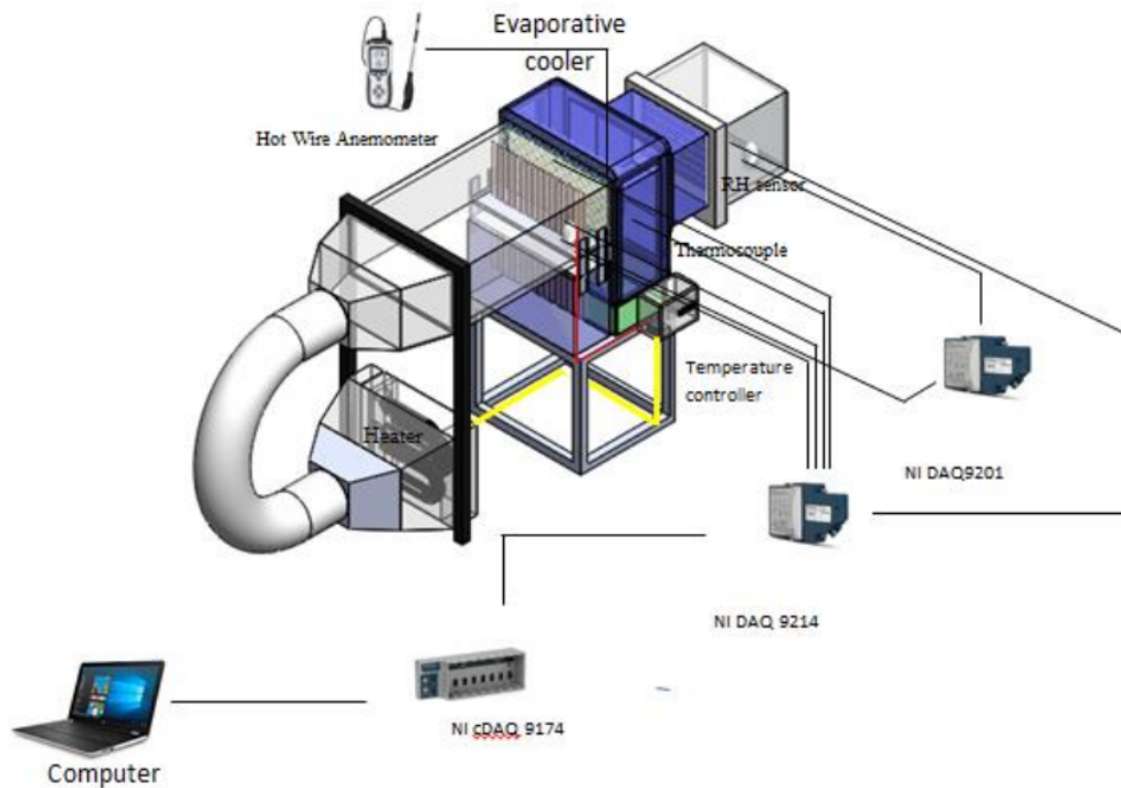
Fig. 3. Schematic of experimental setup
