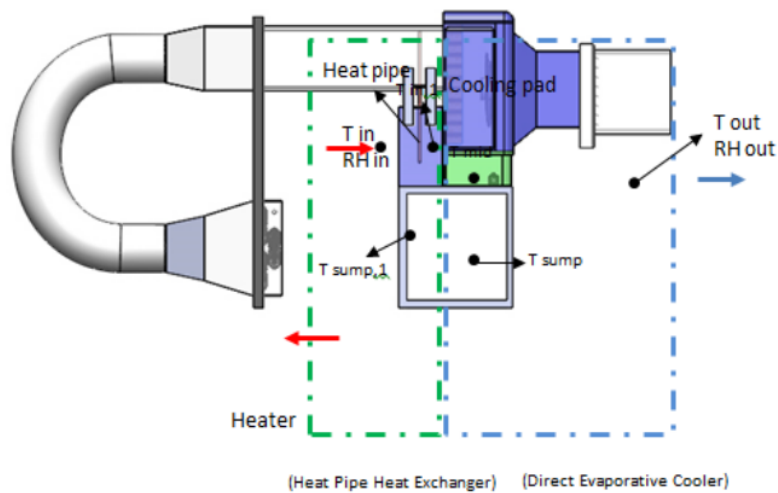
Fig. 2. Schematic of modified direct evaporative cooler
