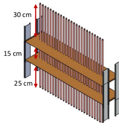
Fig. 1. Heat pipes dimension and configuration
