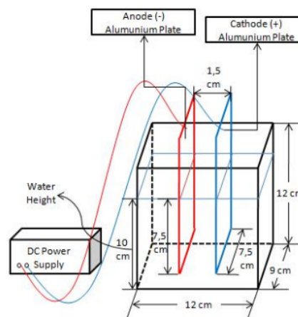
Fig 2. Electrocoagulation reactor design [8].
