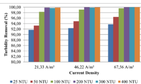
Fig 4. Processing efficiency at any variety of turbidity
