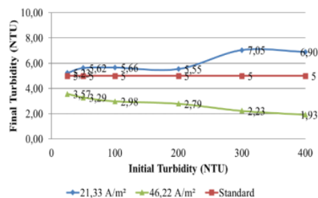
Fig. 5 Decrease of turbidity with initial precipitation and electrocoagulation
