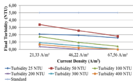
Fig.3 Turbidity removal at each variety of Current Density
