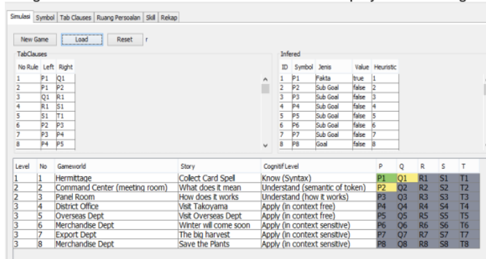
Figure 8 Capture of Engine Implementation for Control Learning State
