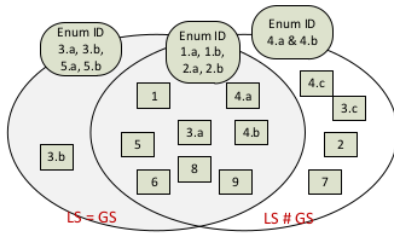
Figure 11 Result of Similarity and Difference analysis
