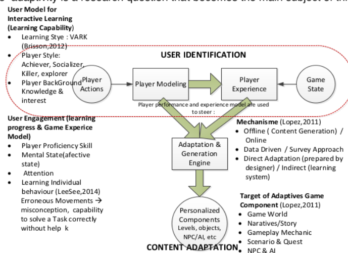
Figure 2 Architecture of Adaptivity in Game – summarized from [1]-[6-10]
