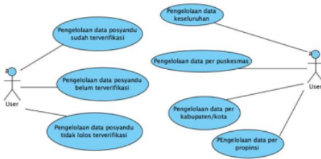
Gambar 7 Diagram use-case iPosyandu
