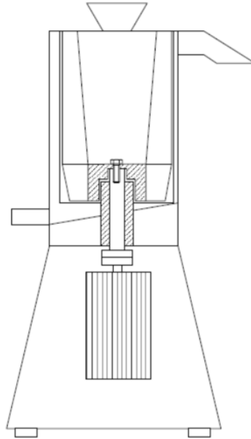
Figure 2. Inside of Pulper
