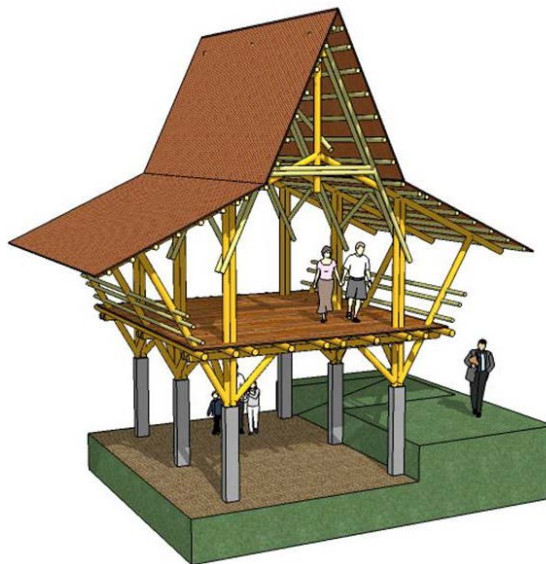
Gambar 2.9 Atap Joglo
