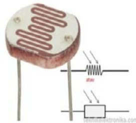
Gambar 2.16 Sensor Cahaya ( LDR )
