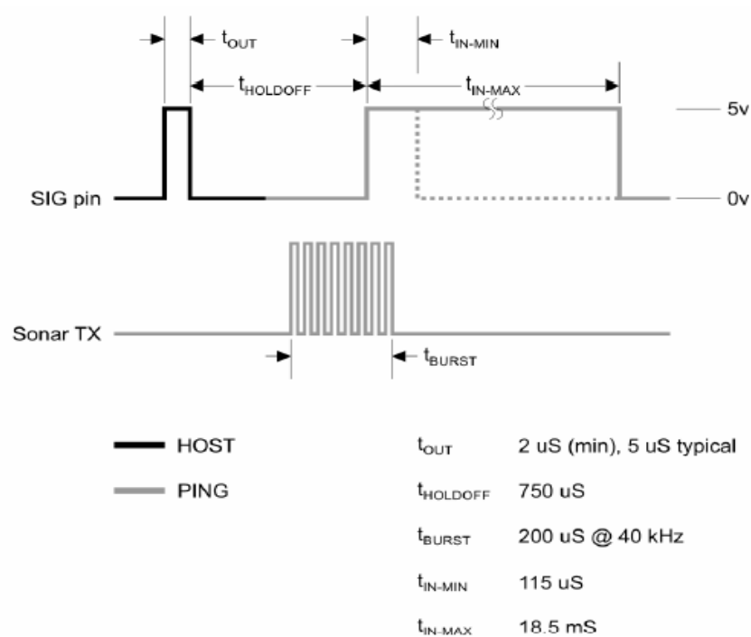
Gambar 3.3 Diagram Waktu Sensor Ultrasonik Ping Parallax
