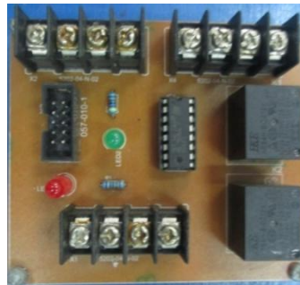
Gambar 3.5 Rangkaian Driver Pompa Air
