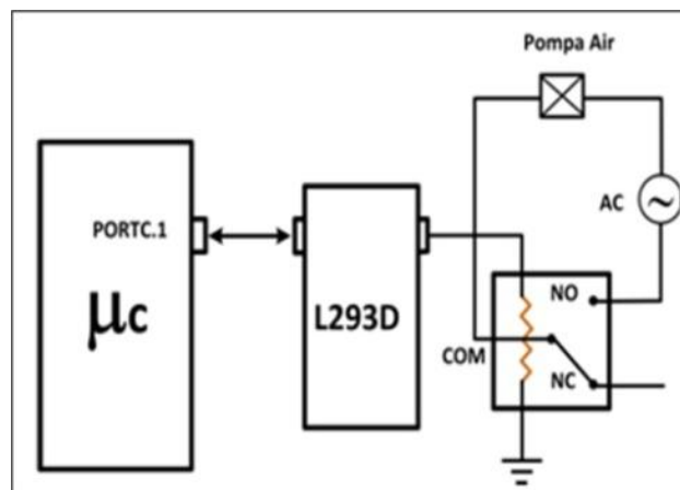
Gambar 4.3 Skematik Driver Pompa Air
