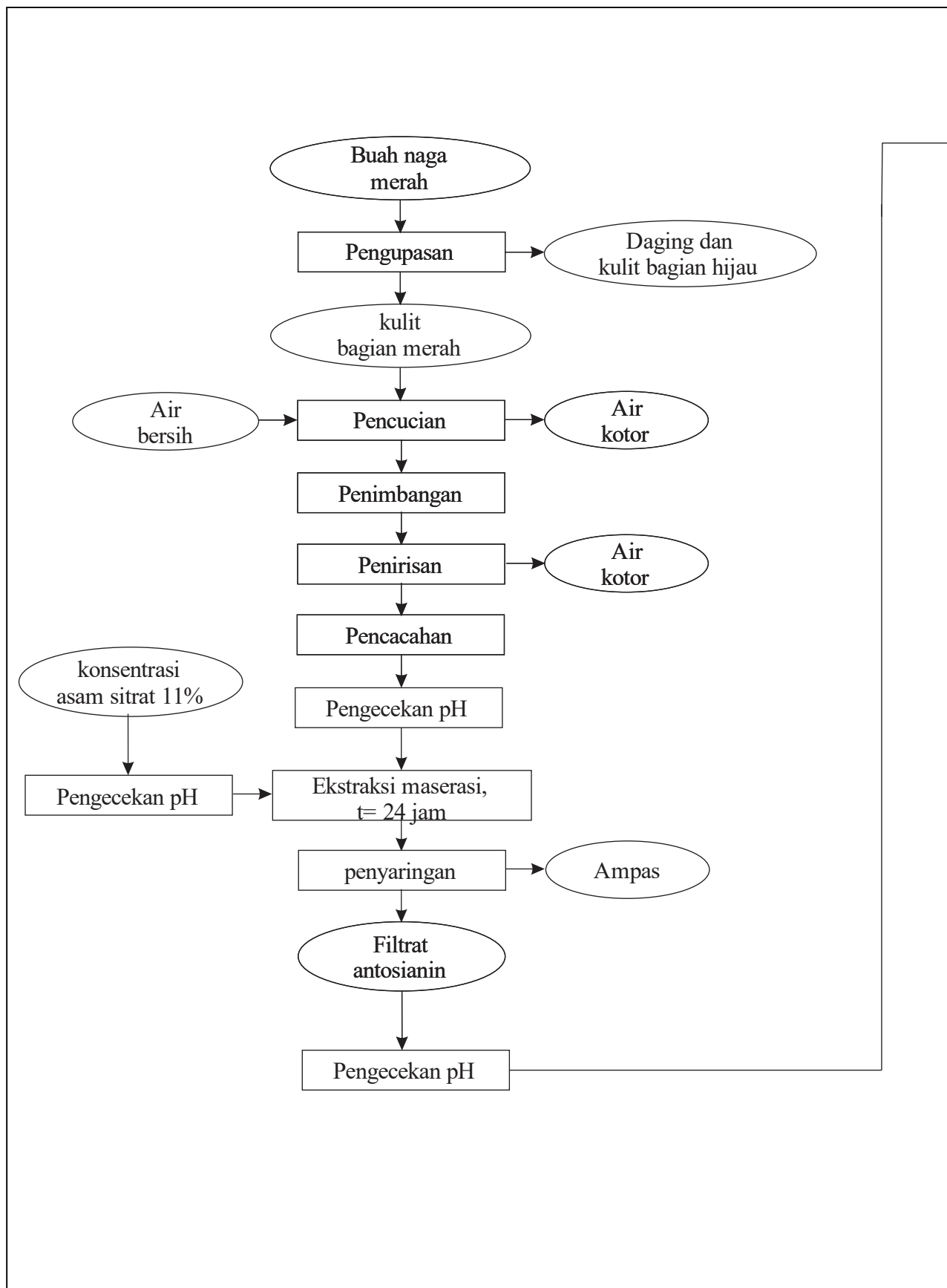
Gambar 4. Diagram Alir
